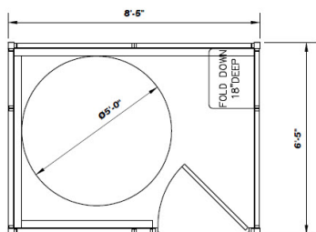
FLOOR PLAN
