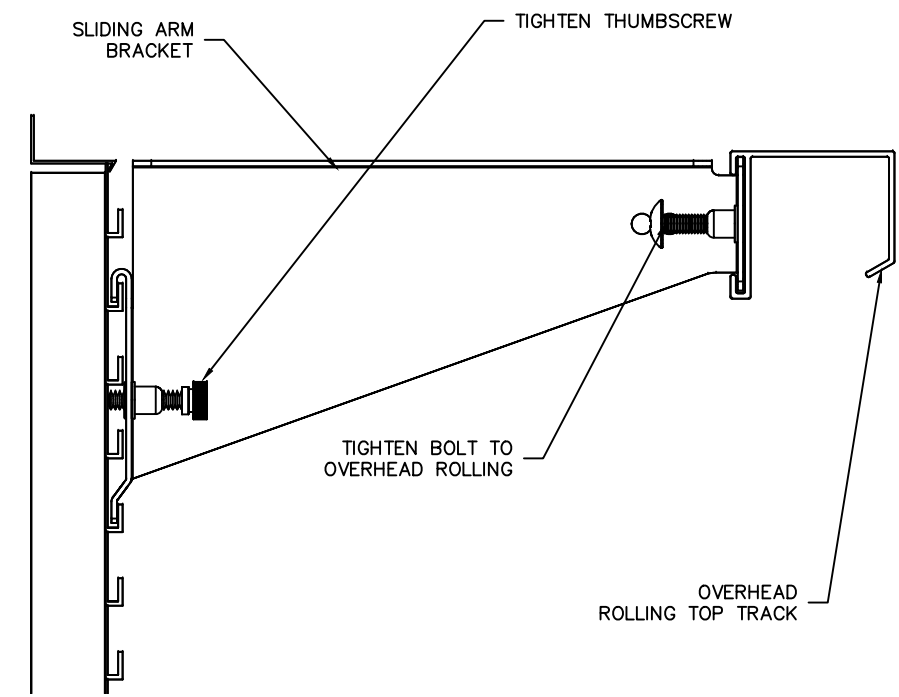
DUAL ARM MOUNT SIDE SECTION VIEW
