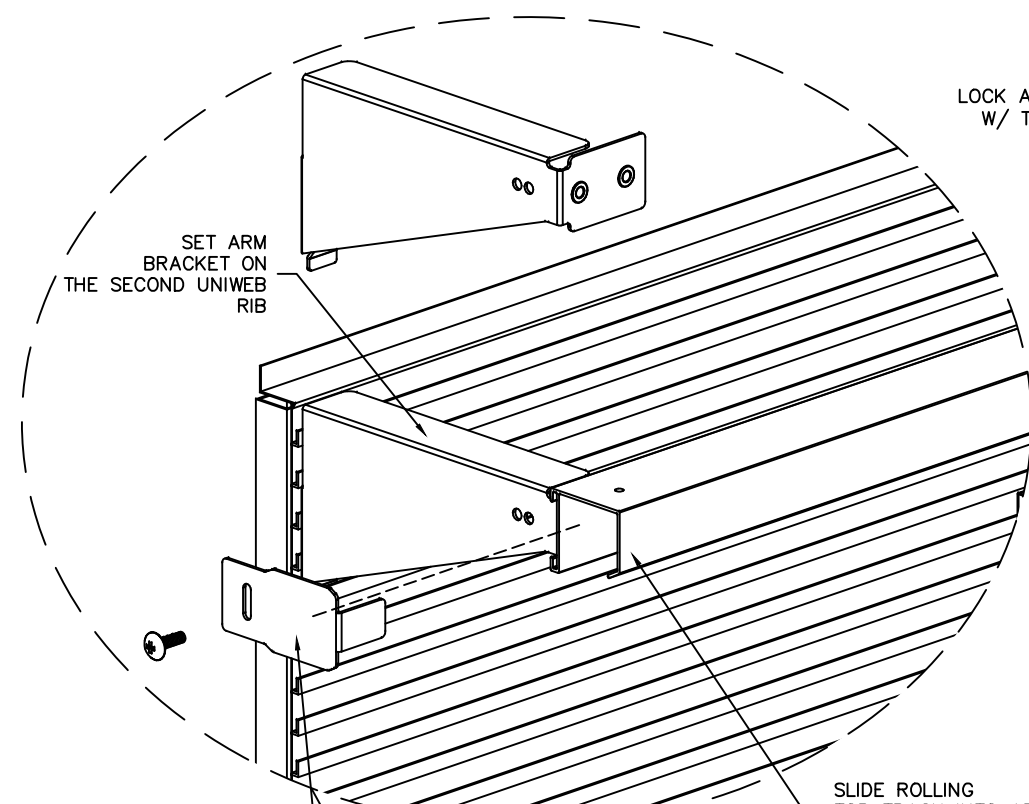
SINGLE ARM MOUNT
