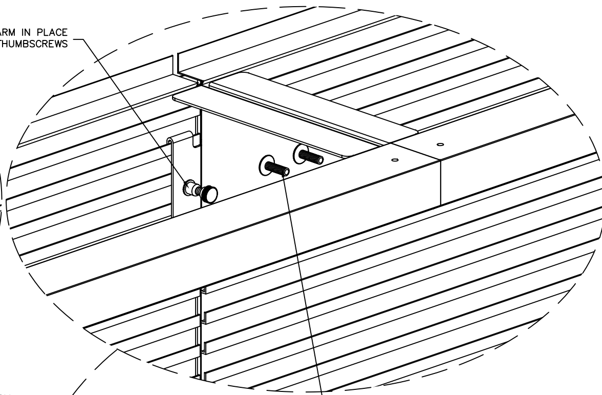
DUAL ARM MOUNT - JOINT
