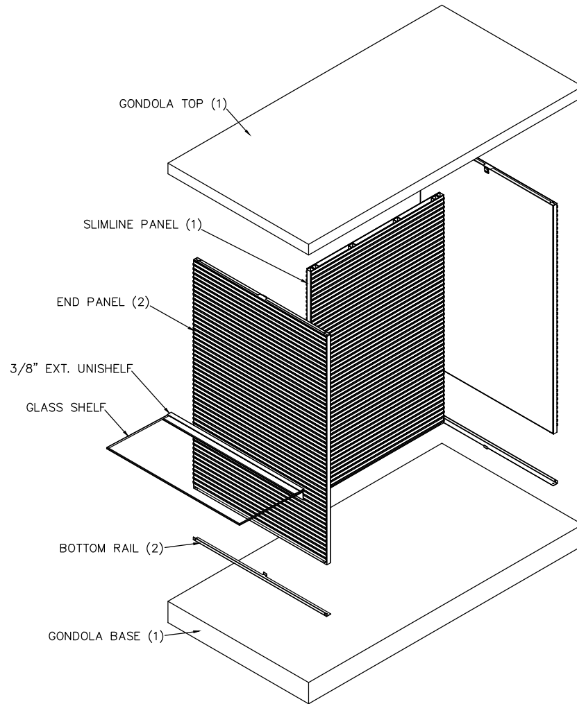
EXPLODED ASSEMBLY VIEW
